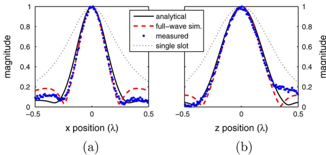
Fig. 4. Comparison of the field profiles along the x -axis (a) and the z -axis (b). Measured data is plotted alongside full-wave simulation data and analytical predictions, with the diffraction limited beam from a single slot given for comparison. The focal plane of the analytic and simulation data was moved to 0.28\lambda so the single-slot data would be consistent with the measurements.
