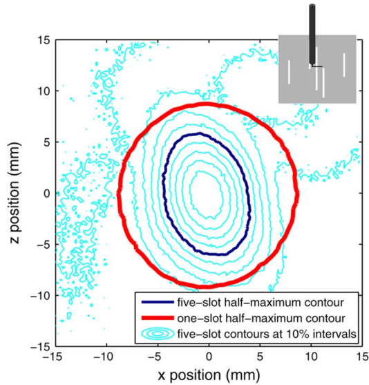
Fig. 3. Experimental measurements of the electric field at 10 GHz over a plane 7.5 mm away from the screen. The thin blue contours are spaced at 10% intervals from 10% to 90% of the peak magnitude while the thicker blue oval contour represents the FWHM focal spot. The thick red round contour represents the FWHM focal spot of the diffraction limited beam produced by a single slot. Asymmetries in the measured field profile were exacerbated by the asymmetric coupling between the probe antenna and the slots (see inset).
