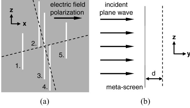
Fig. 1. (a) Geometry of the slotted meta-screen showing the numbering of the slots from one to five. The slots are arranged along orthogonal focusing axes with their centers equidistant from the origin to provide 2-D focusing. (b) The meta-screen orientation with respect to the incident field. The electric field is polarized along the x -direction with the focal plane parallel to the screen but separated by a distance d .
