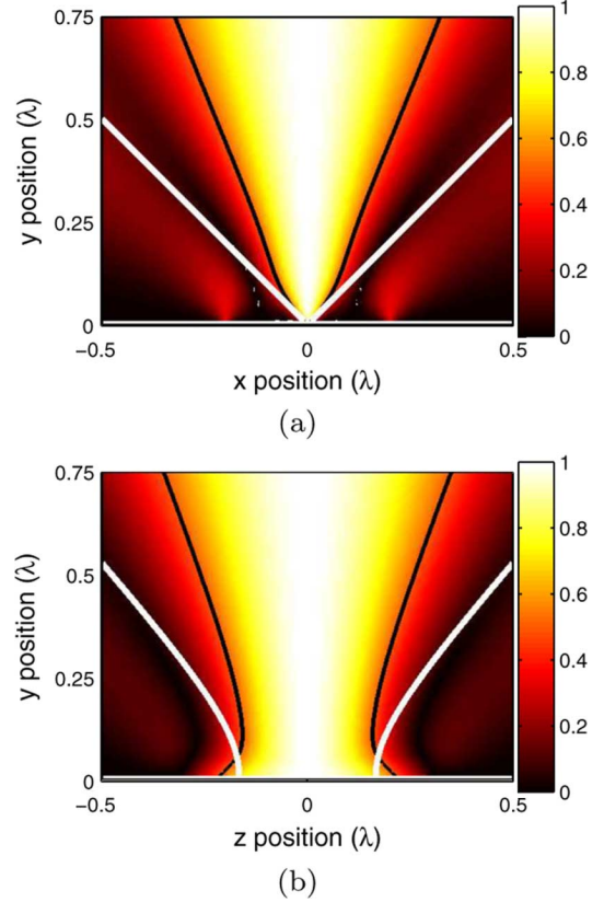
Fig. 2. Full-wave simulations of the electric field magnitude emanating from the meta-screen under plane wave excitation. The fields are normalized transverse to the y -axis at every y position to highlight the profile of the beam as it progresses away from the screen. The xy -plane is shown in (a) with the zy -plane in (b). The thinner black contour indicates the FWHM beam width of the focused beam while the thick white contour indicates the FWHM beam width of a single slot.
