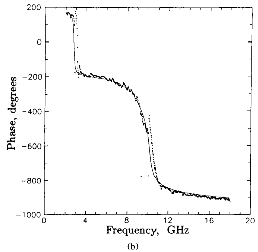
Fig. 7. Measured (dots) and theoretical (solid line) phase of the reflection coefficient for the (a) inductive grid and (b) capacitive grid. Note that the two phase scales are quite different.
