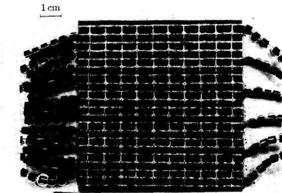
Fig. 1. The 100-MESFET planar grid oscillator. The horizontal lines are the bias lines. Ferrite beads are added to the bias lines to suppress low-frequency oscillations. All the gates, drains, and sources are connected, so there are a total of three wires used for the grid bias. The vertical leads are gates and drains and the radiated electric field is polarized in this direction.
